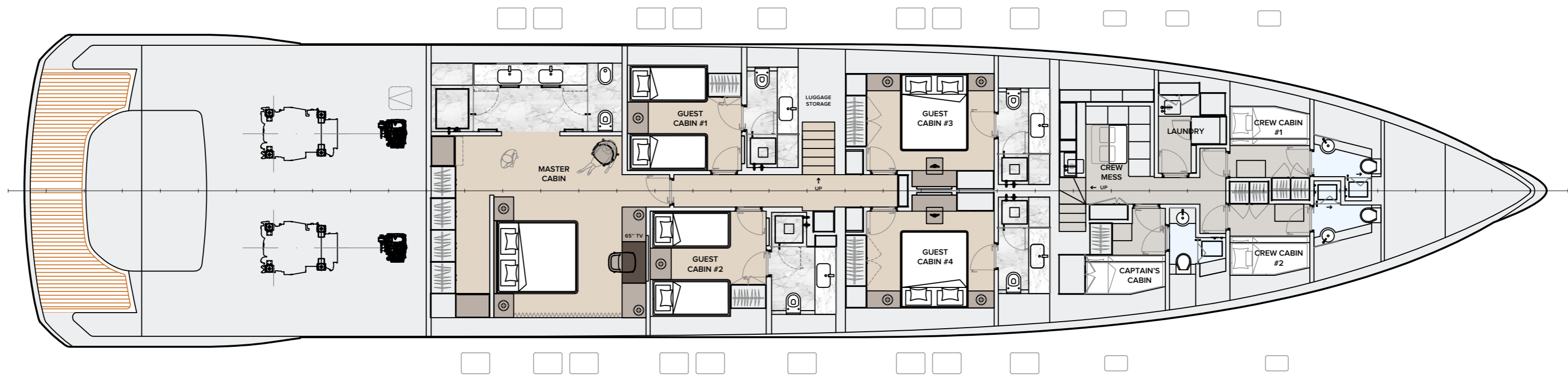
LOWER DECK
