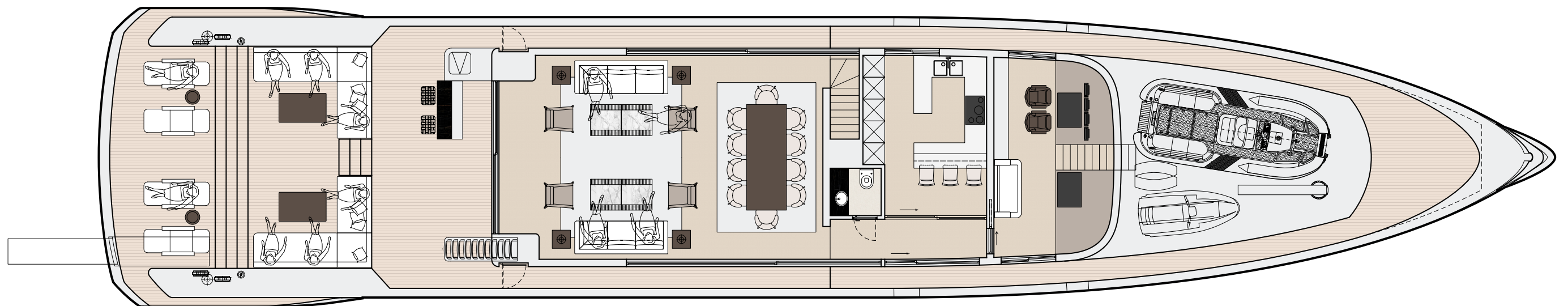
Main deck
